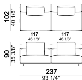
Central unit
